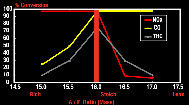
3-Way Catalyst Performance Curve
